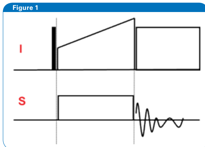
Displays the basic cross polarization experiment. Our experiment used the amplitude ramp on the I spin and always from low to high amplitude, as shown, although equivalent performance may be obtained by instead inverting its slope and/or applying to the S spin with constant amplitude on I. The open rectangle following the ramped pulse on channel I represents any decoupling pulse sequence, while the filled rectangular pulse is a 90^\circ excitation pulse for I spins, which are ^1\text{H} spins in our case.
